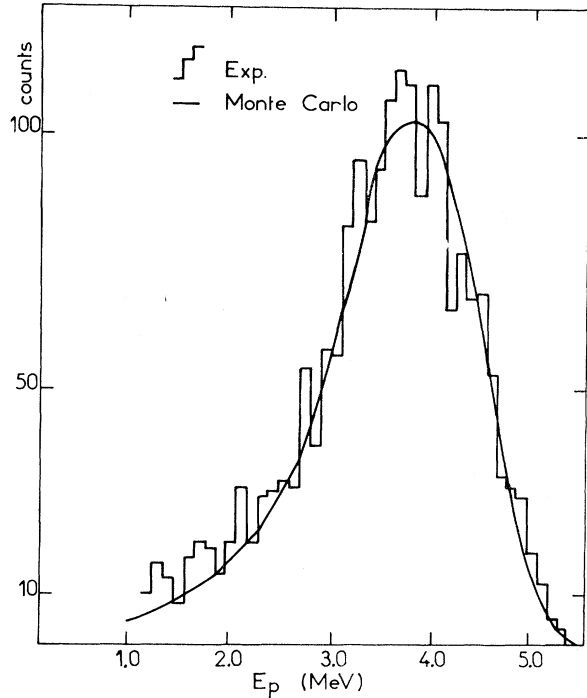
FIG. 9. Typical energy spectrum obtained in coincidence between the two analyzers with a 29-mg/cm 2 carbon target. Accidental coincidences have been subtracted.
